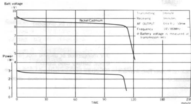
Fig. 1-1 Operating time
